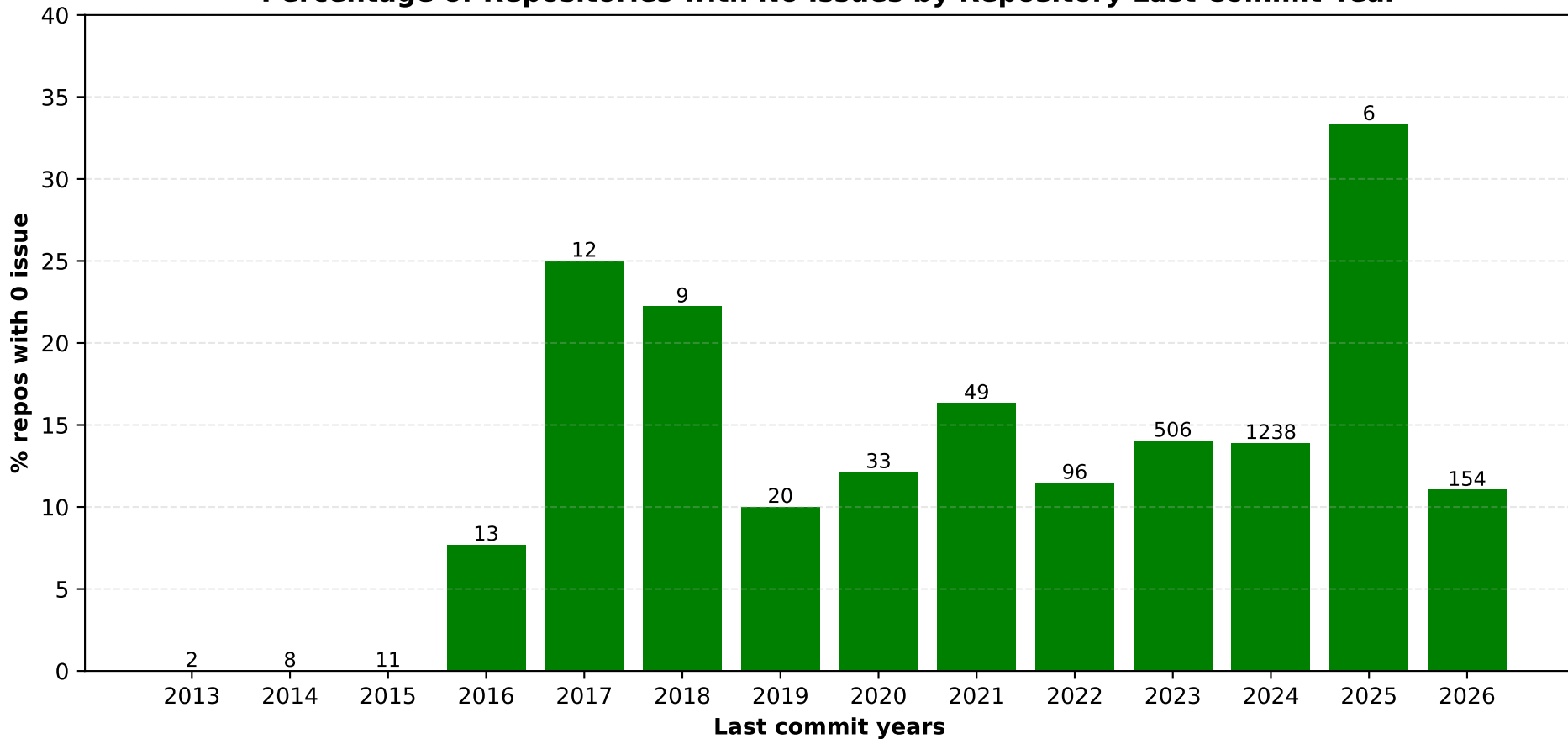
Percentage of Repositories with No Issues by Repository Last Commit Year
